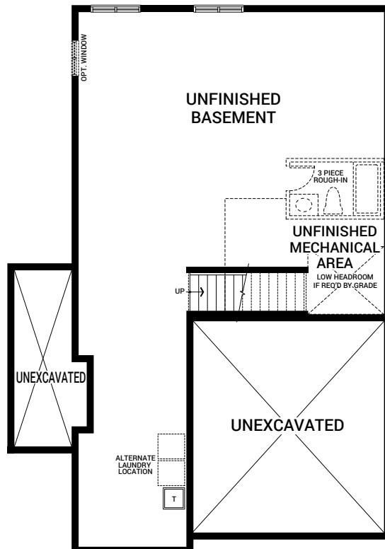
BASEMENT FLOOR PLAN C
