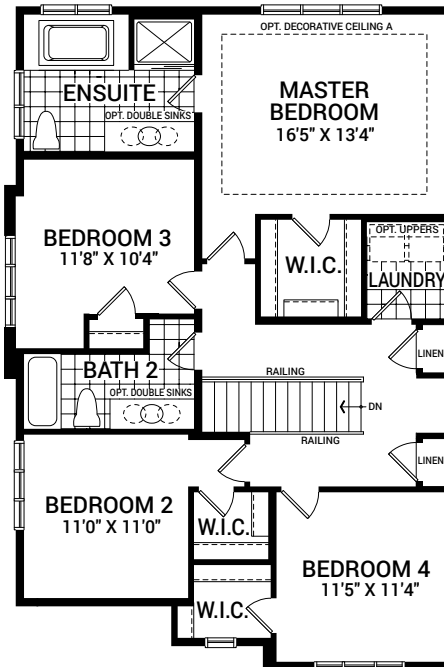
SECOND FLOOR PLAN C
