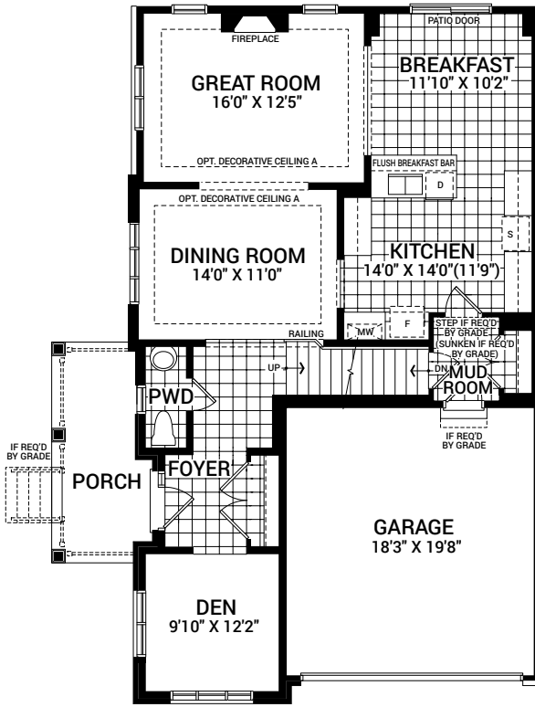
MAIN FLOOR PLAN C
