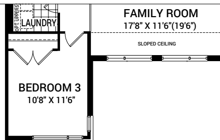
SECOND FLOOR PLAN B
