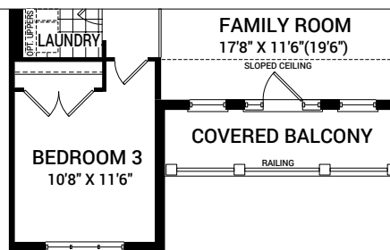
SECOND FLOOR PLAN C
