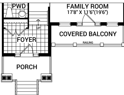
MAIN FLOOR PLAN C
