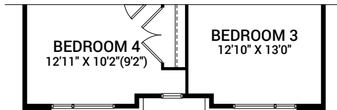
SECOND FLOOR PLAN B
