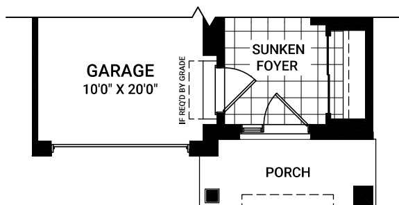
FIRST FLOOR ELEVATION B
