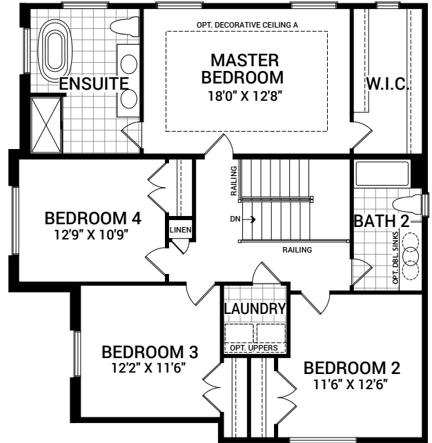
SECOND FLOOR PLAN C
