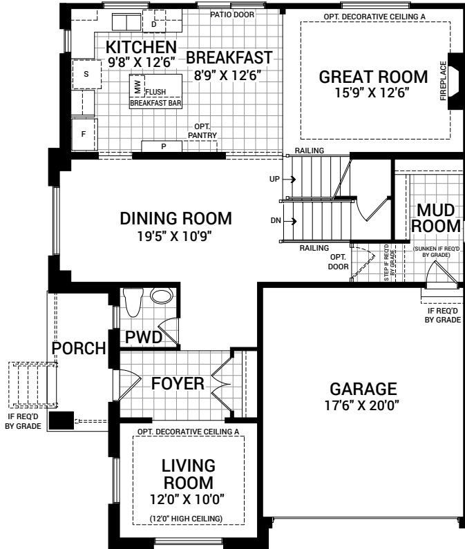
MAIN FLOOR PLAN C
