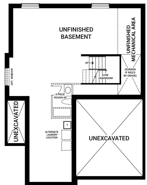
BASEMENT PLAN A & B
