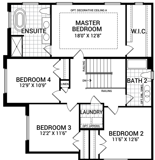
SECOND FLOOR PLAN B
