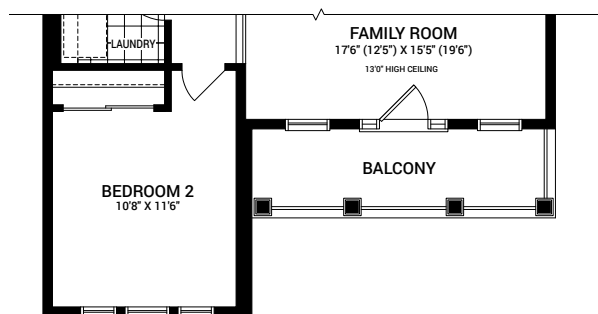
SECOND FLOOR PLAN B
