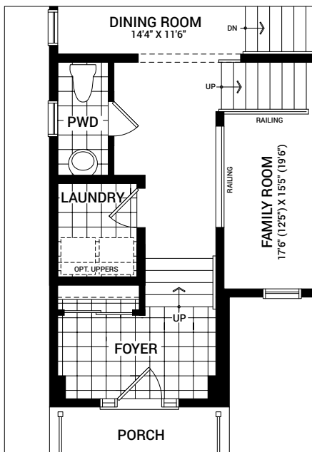
OPTIONAL MAIN FLOOR LAUNDRY LAYOUT A
