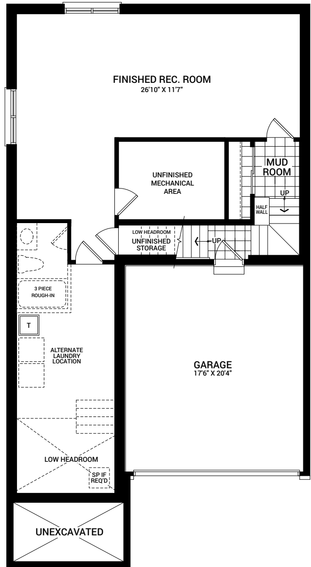
OPTIONAL FINISHED BASEMENT REC. ROOM
