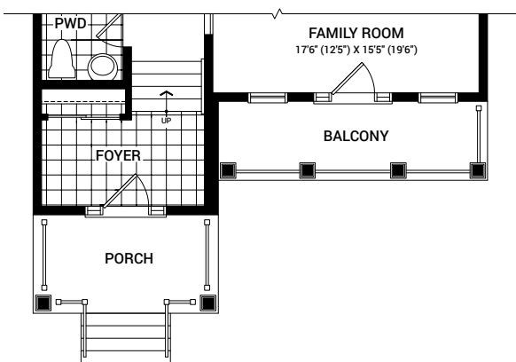
MAIN FLOOR PLAN B
