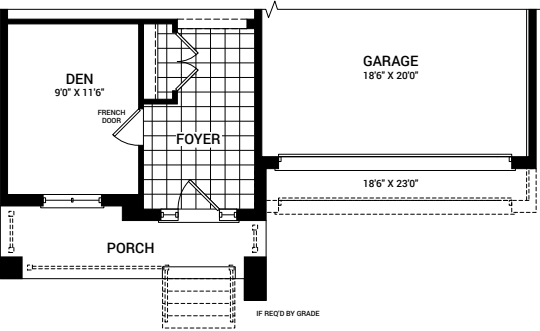
MAIN FLOOR PLAN D
