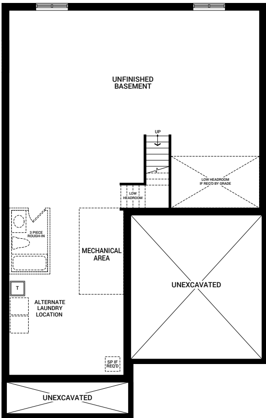
BASEMENT FLOOR PLAN A (SIMILAR FOR PLAN C & D)
