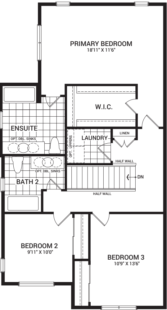
SECOND FLOOR
