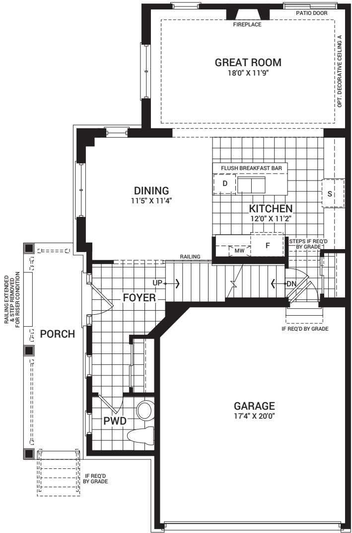
MAIN FLOOR
