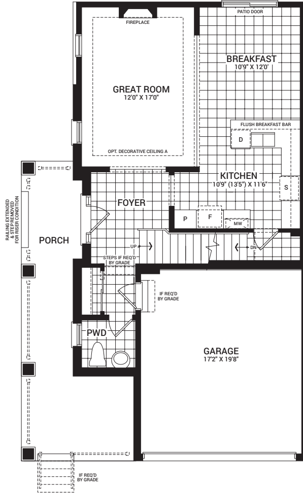
MAIN FLOOR PLAN B
