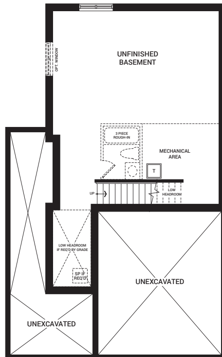
BASEMENT FLOOR PLAN B
