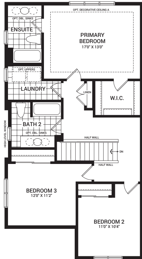
SECOND FLOOR PLAN A 3 BEDROOM PLAN
