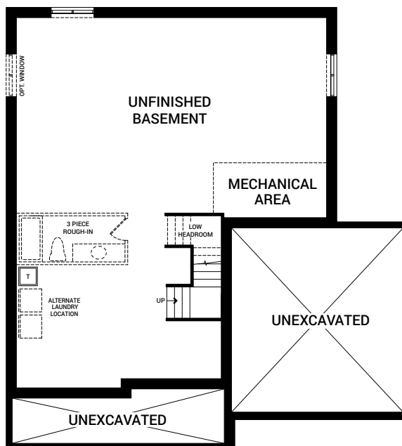
BASEMENT PLAN A (SIMILAR FOR PLAN B & C)
