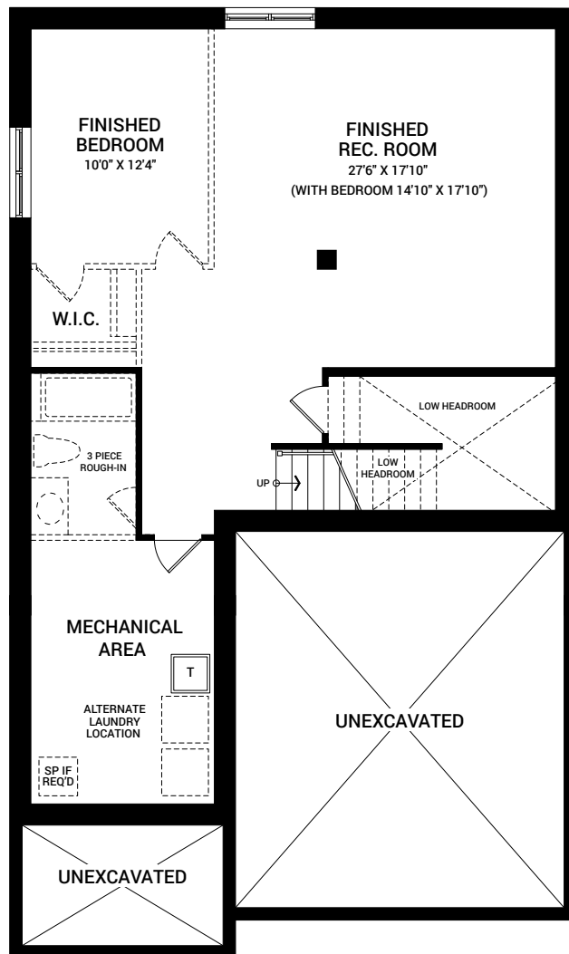
OPTIONAL FINISHED BASEMENT REC. ROOM W/ OPTIONAL BEDROOM (SIMILAR FOR PLAN B & C)
