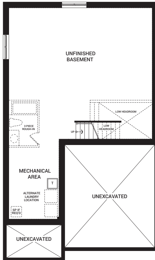
BASEMENT PLAN A, B & C
