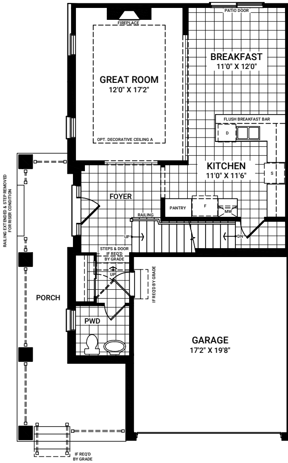
FIRST FLOOR ELEVATION B
