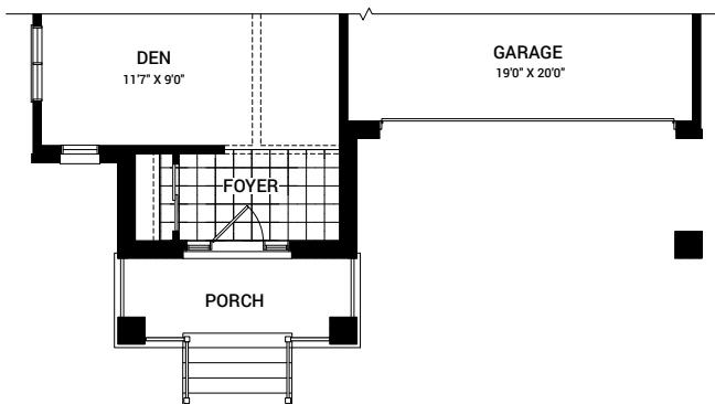
MAIN FLOOR PLAN C
