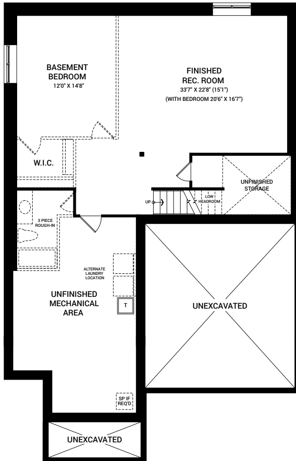
FINISHED BASEMENT FLOOR PLAN
