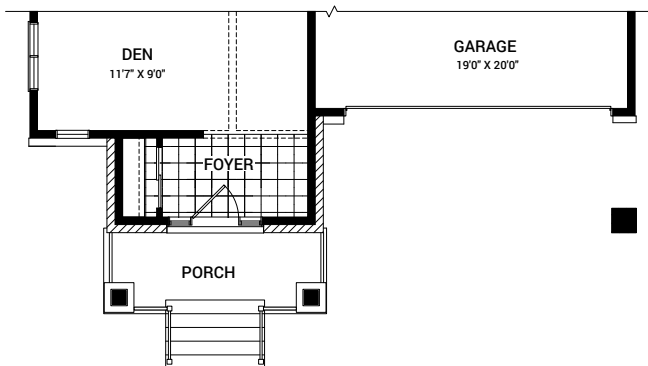
MAIN FLOOR PLAN B
