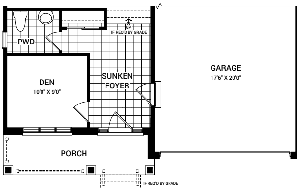
MAIN FLOOR PLAN C
