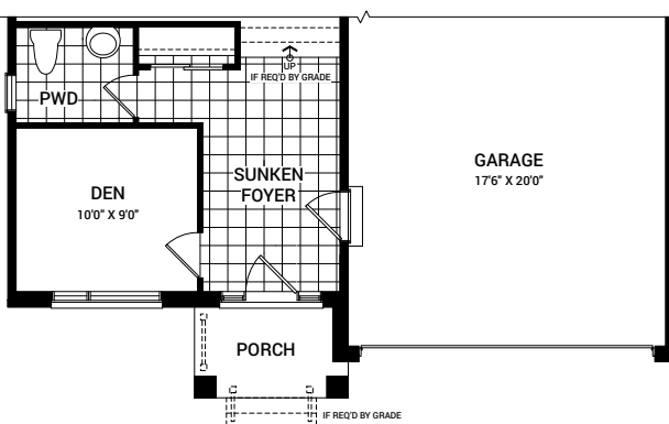
MAIN FLOOR PLAN B
