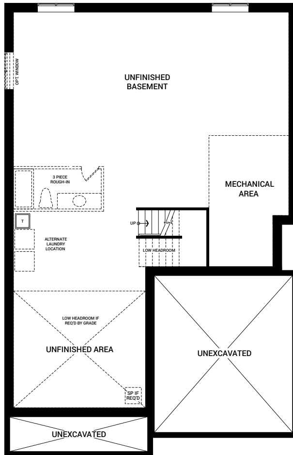
BASEMENT FLOOR PLAN A (SIMILAR FOR PLAN B & C)
