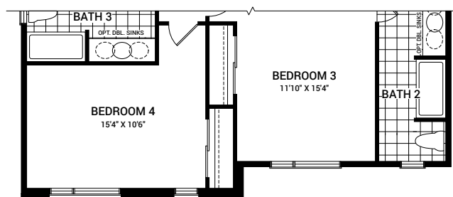
SECOND FLOOR PLAN B
