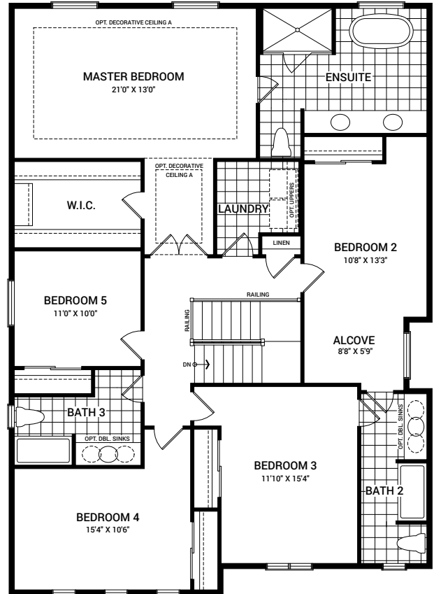
SECOND FLOOR PLAN A
