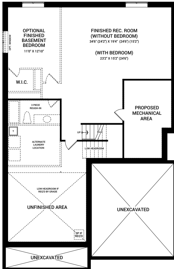
OPTIONAL FINISHED BASEMENT REC. ROOM W/OPTIONAL BEDROOM (SIMILAR FOR PLAN B & C)
