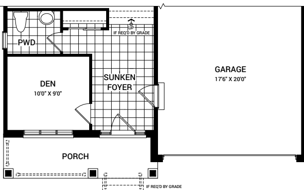
MAIN FLOOR PLAN C
