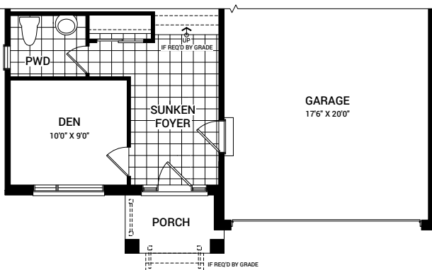
MAIN FLOOR PLAN B
