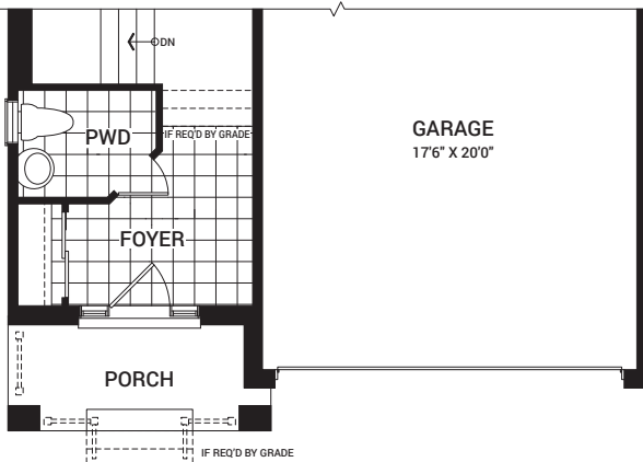
MAIN FLOOR PLAN B
