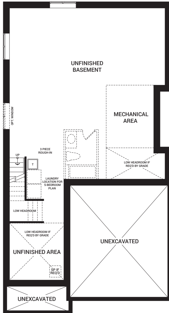
BASEMENT FLOOR PLAN A (SIMILAR FOR PLAN B & C)
