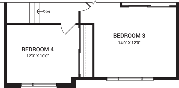
SECOND FLOOR PLAN B
