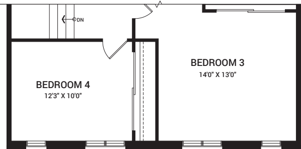
SECOND FLOOR PLAN C
