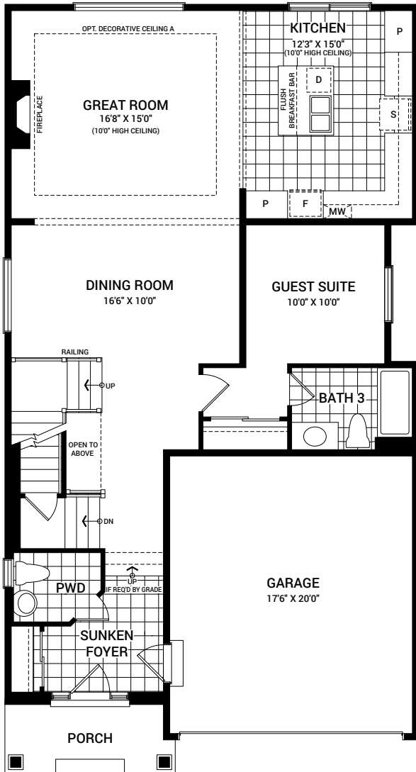
OPTIONAL MAIN FLOOR PLAN A
