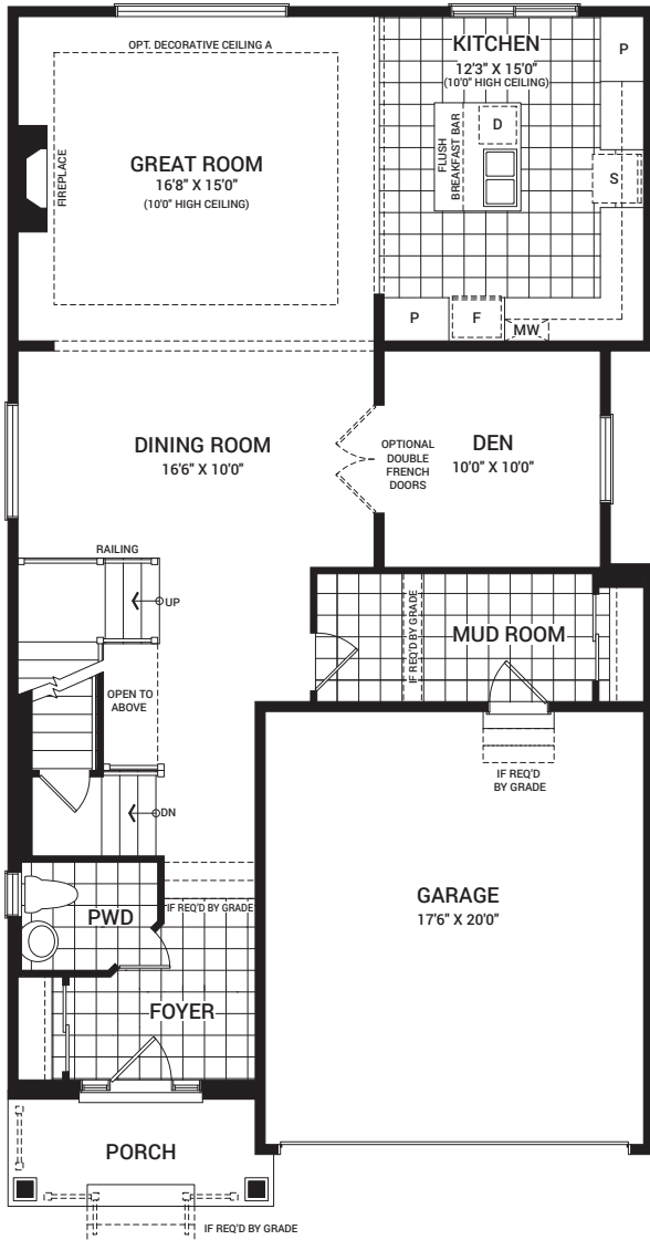
MAIN FLOOR PLAN A
