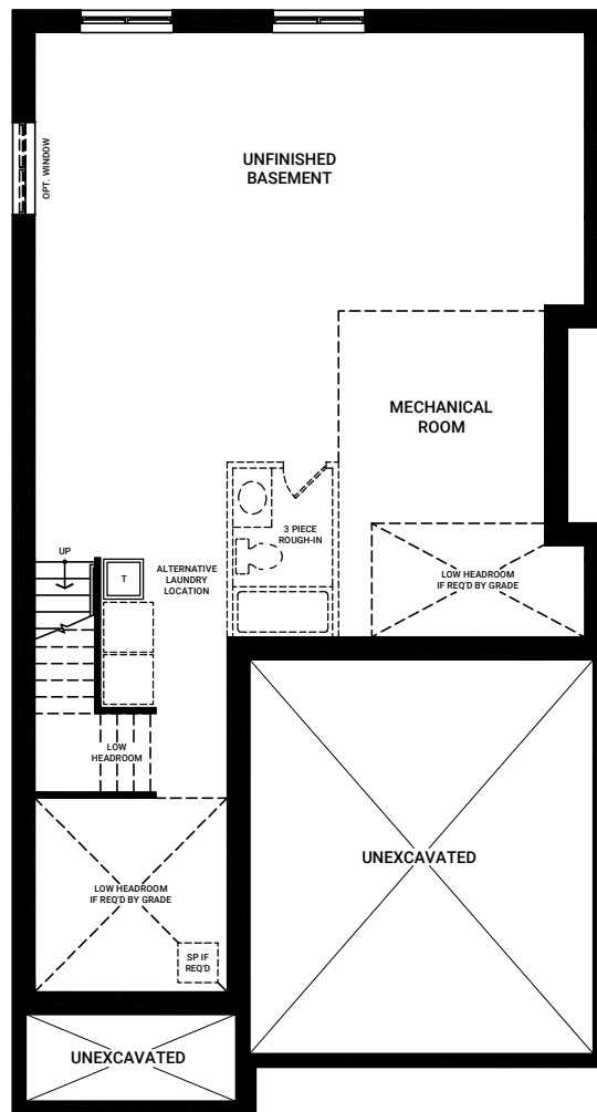
BASEMENT FLOOR ELEVATION A (SIMILAR FOR ELEVATIONS B, C & E)
