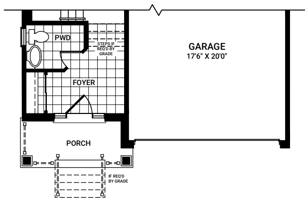
FIRST FLOOR ELEVATION B
