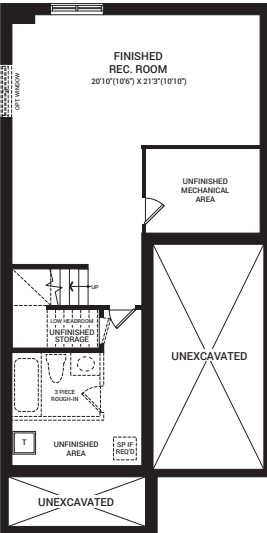
OPTIONAL FINISHED BASEMENT REC. ROOM
