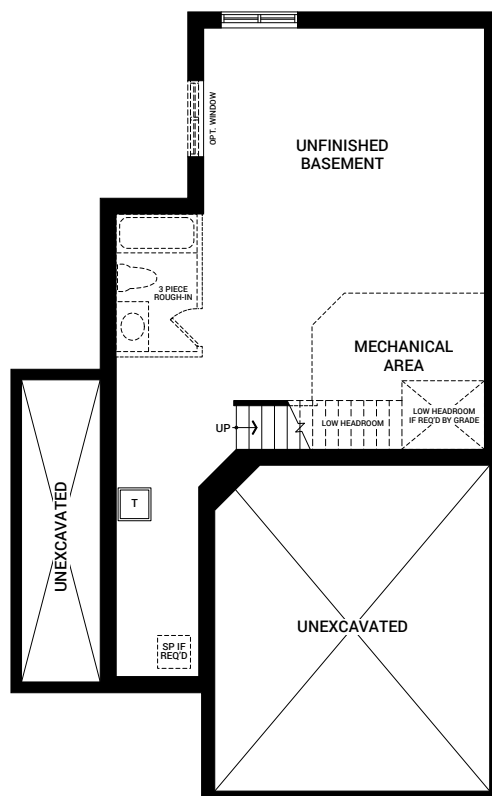
BASEMENT FLOOR PLAN A
