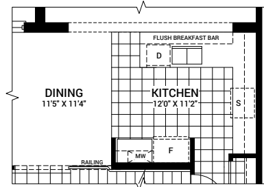
OPTIONAL KITCHEN LAYOUT A
