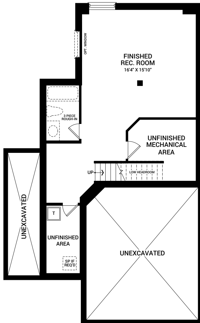
OPTIONAL FINISHED BASEMENT REC. ROOM
