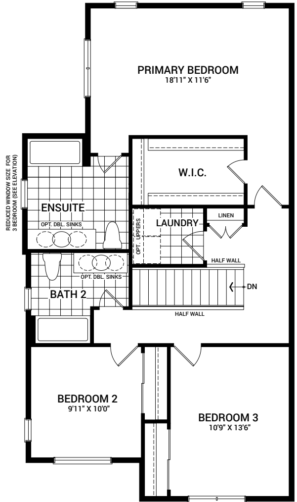
SECOND FLOOR PLAN A
