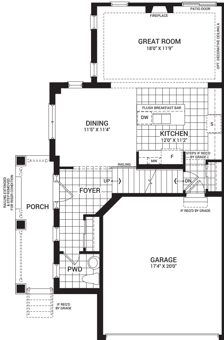
MAIN FLOOR PLAN B
