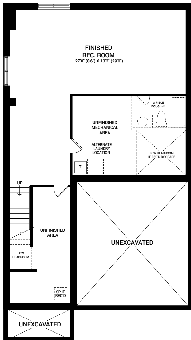
OPTIONAL FINISHED BASEMENT REC. ROOM
