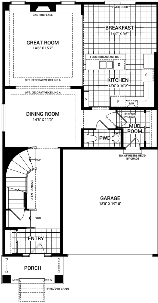
MAIN FLOOR PLAN A
