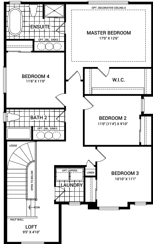
SECOND FLOOR PLAN A
