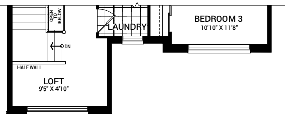
SECOND FLOOR PLAN D
