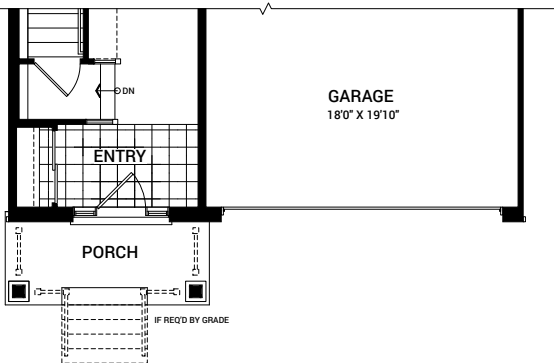
MAIN FLOOR PLAN B
