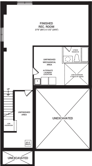
OPTIONAL FINISHED BASEMENT REC. ROOM
