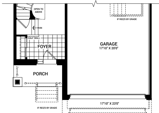
MAIN FLOOR PLAN C
