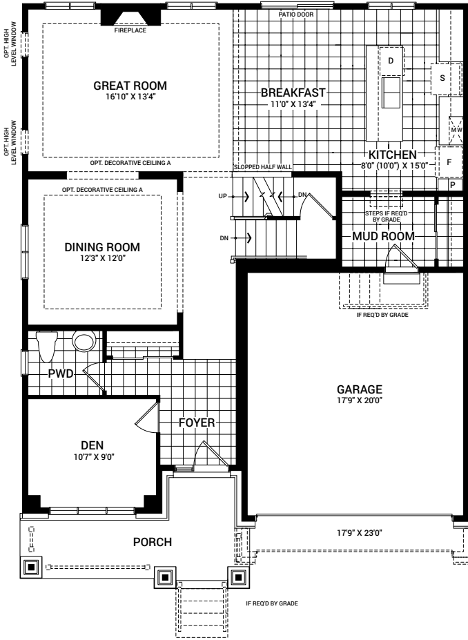
MAIN FLOOR PLAN A
