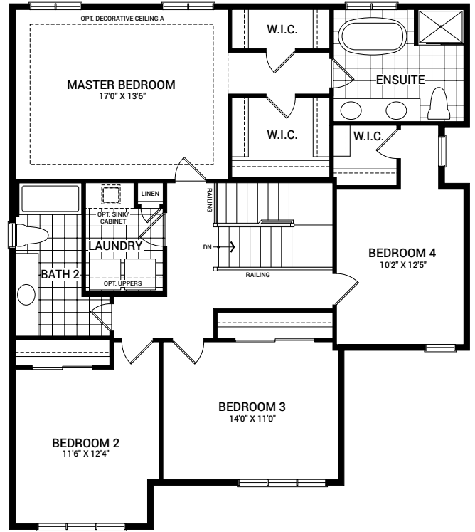
SECOND FLOOR PLAN A
