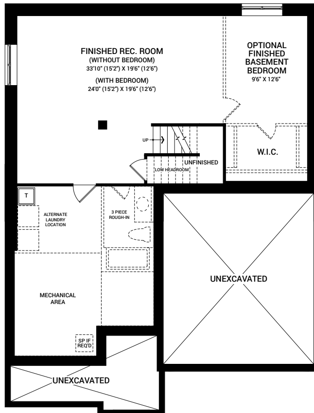
OPTIONAL FINISHED BASEMENT REC. ROOM W/ OPTIONAL BEDROOM (SIMILAR FOR PLANS B & C)
