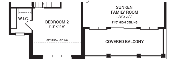
SECOND FLOOR PLAN B
