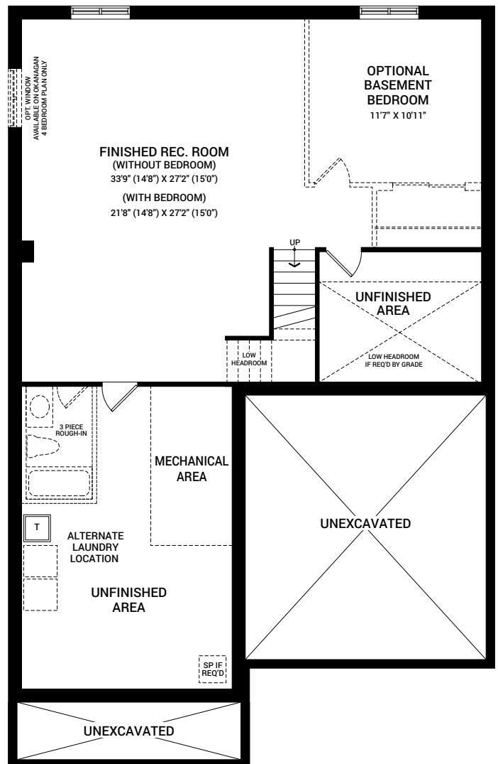
OPTIONAL FINISHED BASEMENT REC. ROOM W/ OPTIONAL BEDROOM (SIMILAR FOR PLAN C & D)
