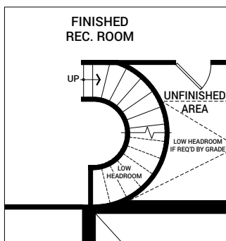
OPTIONAL CIRCULAR BASEMENT STAIR (UNFINISHED)
