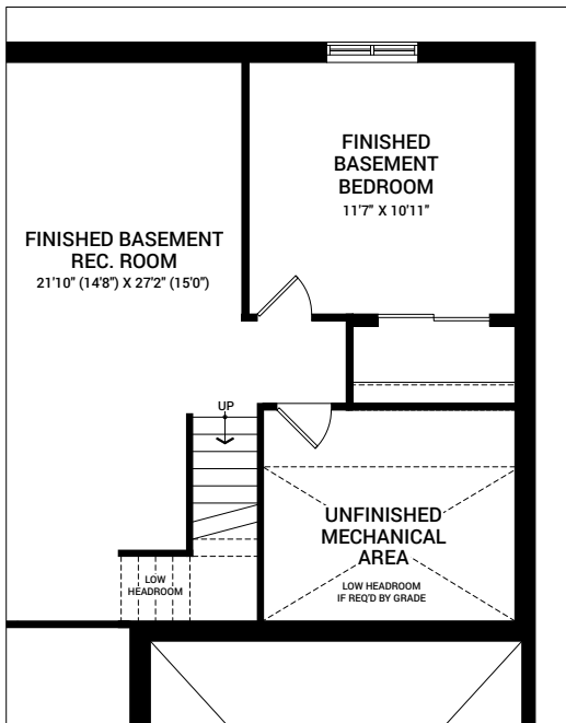
OPTIONAL FINISHED BASEMENT BEDROOM
