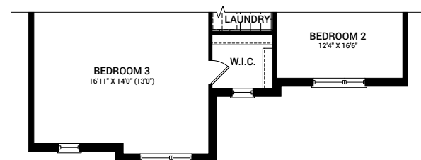
SECOND FLOOR PLAN D
