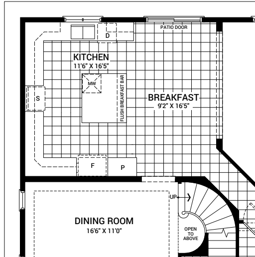
OPTIONAL KITCHEN LAYOUT B
