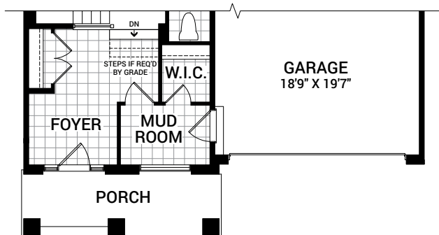
MAIN FLOOR PLAN C
