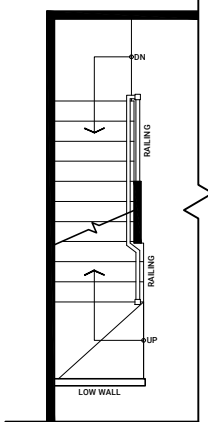
LOW WALL TO RAILING
