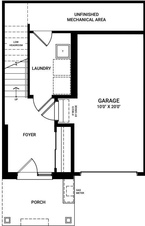
FIRST FLOOR ELEVATION A (SIMILAR FOR ELEVATION B)
