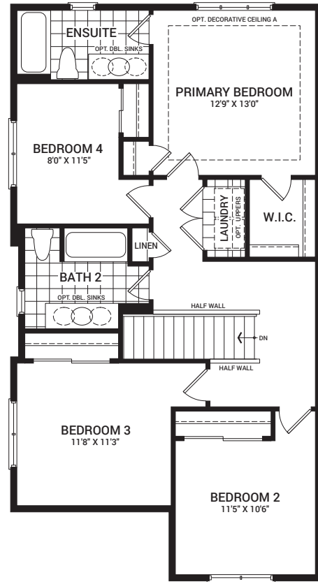
SECOND FLOOR PLAN A 4 BEDROOM
