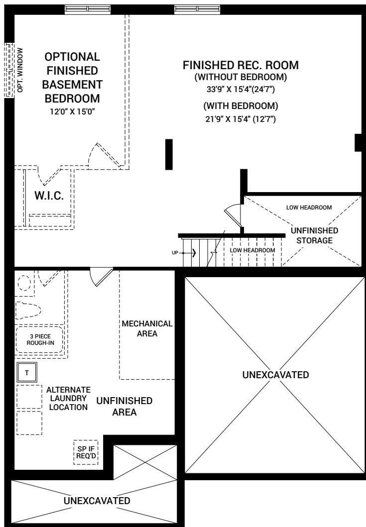
OPTIONAL FINISHED BASEMENT REC. ROOM W/ OPTIONAL BEDROOM
