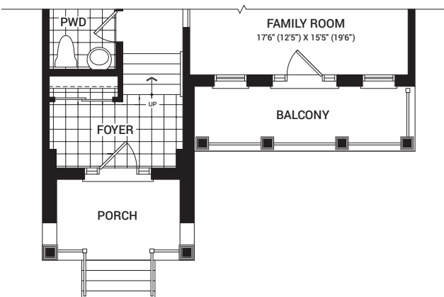
MAIN FLOOR PLAN C
