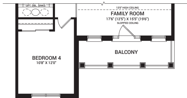
SECOND FLOOR PLAN C
