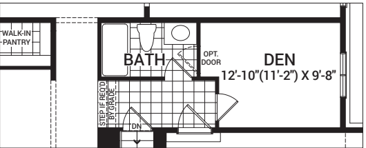
OPTIONAL MAIN FLOOR LAYOUT B
