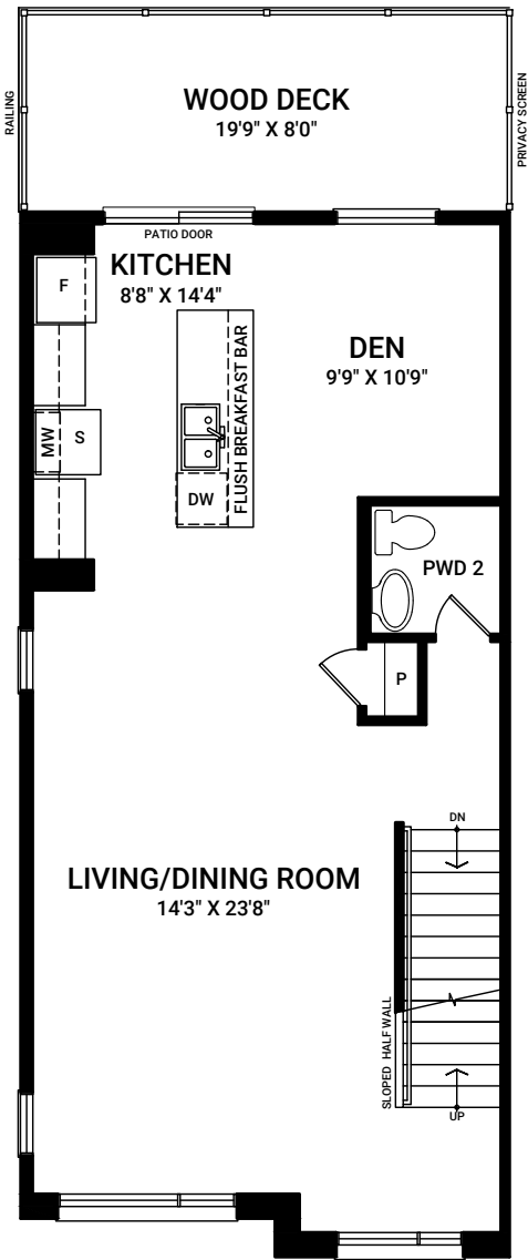
SECOND FLOOR PLAN A END CONDITION
