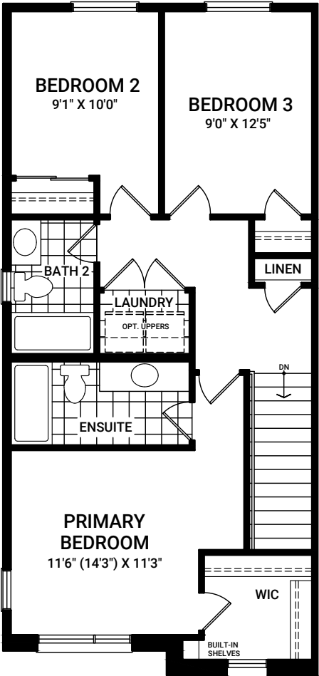
THIRD FLOOR PLAN A END CONDITION
