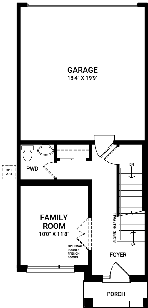
FIRST FLOOR PLAN A END CONDITION
