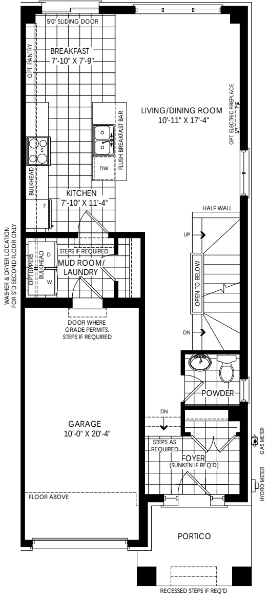
GROUND FLOOR PLAN ELEV. 'A'
