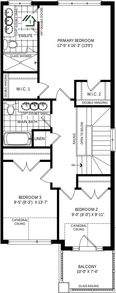
SECOND FLOOR PLAN ELEV. 'A'
