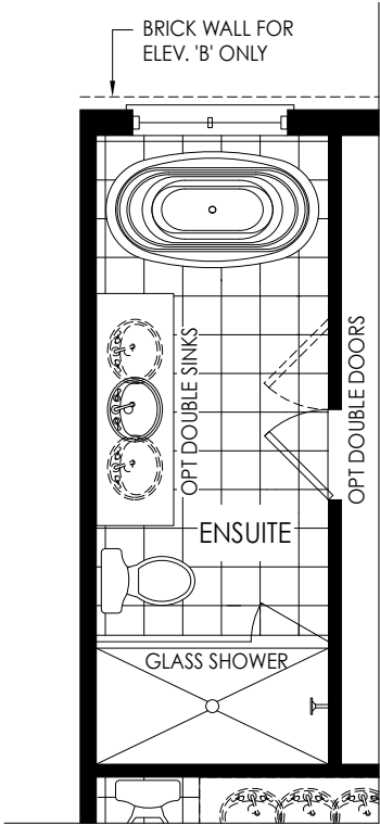
PARTIAL OPT. SECOND FLOOR PLAN ELEV. 'A' & 'B' W/ ALT. PRIMARY ENSUITE
