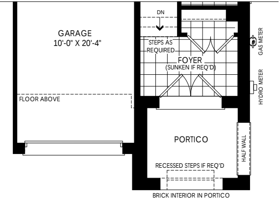
PARTIAL GROUND FLOOR PLAN ELEV. 'B'
