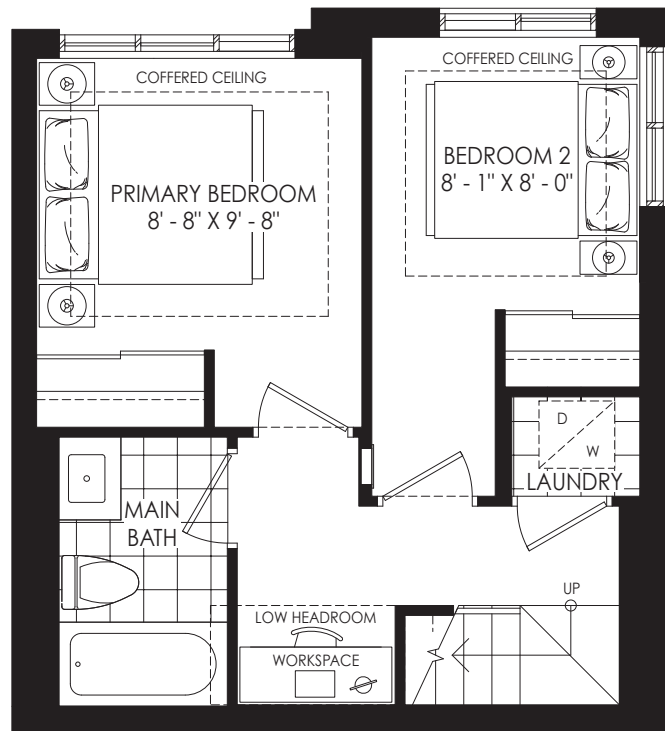
FOURTH FLOOR
