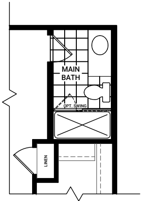
PRE-FAB BASE
