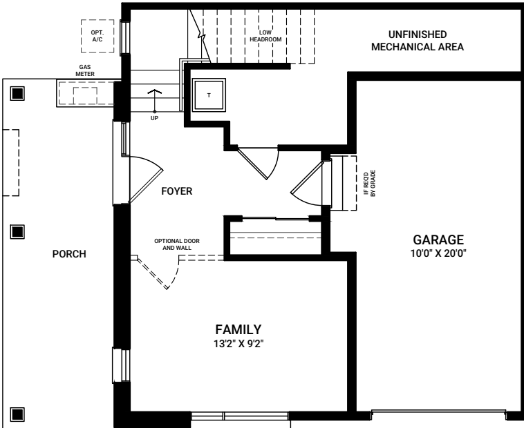
FIRST FLOOR ELEVATION A (SIMILAR FOR ELEVATION B)
