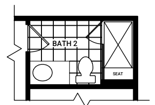
BATH 2 TUB TO 4 ft SHOWER PLUS BENCH
