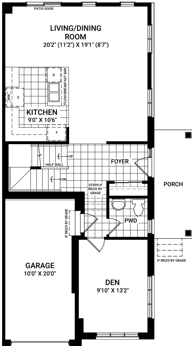
FIRST FLOOR ELEVATION A
