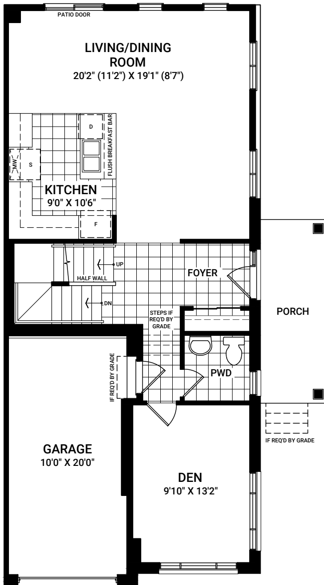
FIRST FLOOR ELEVATION B
