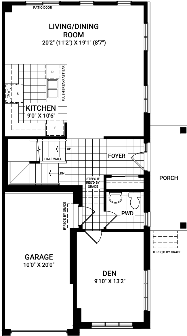
FIRST FLOOR ELEVATION C
