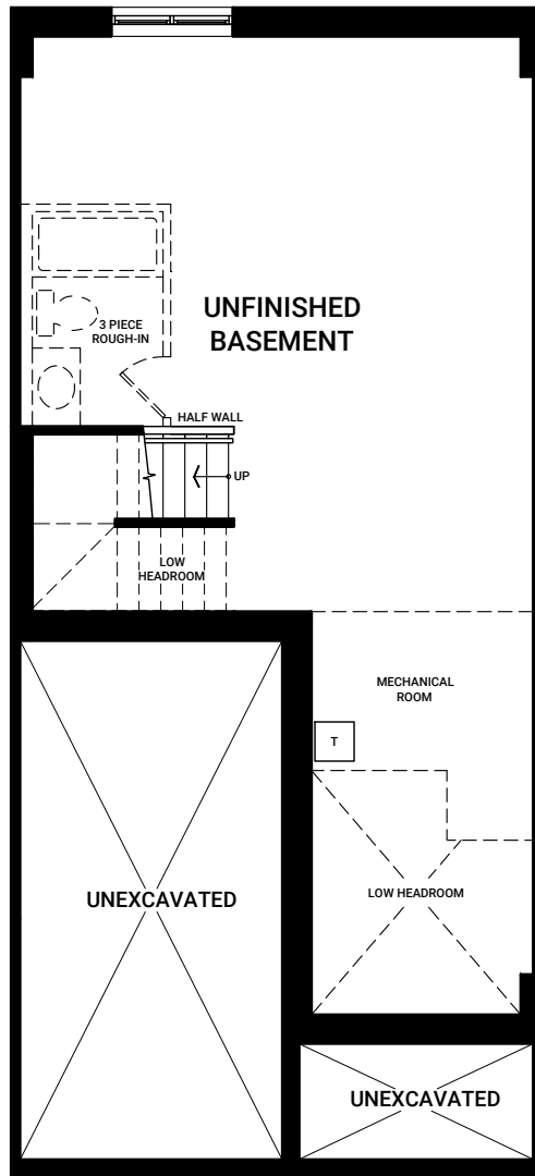
BASEMENT ELEVATION A (SIMILAR FOR ELEVATIONS B & C)
