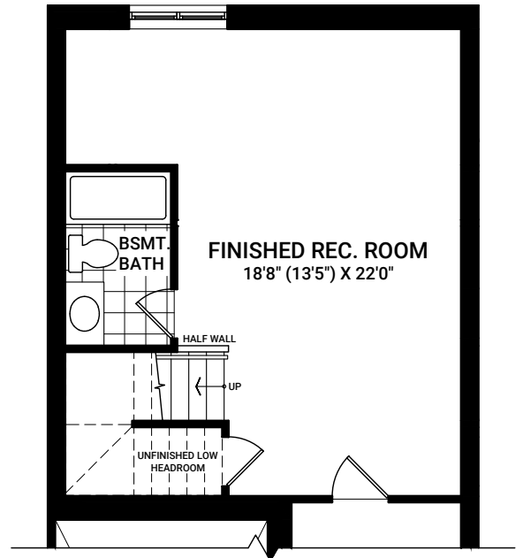
OPTIONAL FINISHED BASEMENT REC. ROOM WITH 3 PIECE BATH
