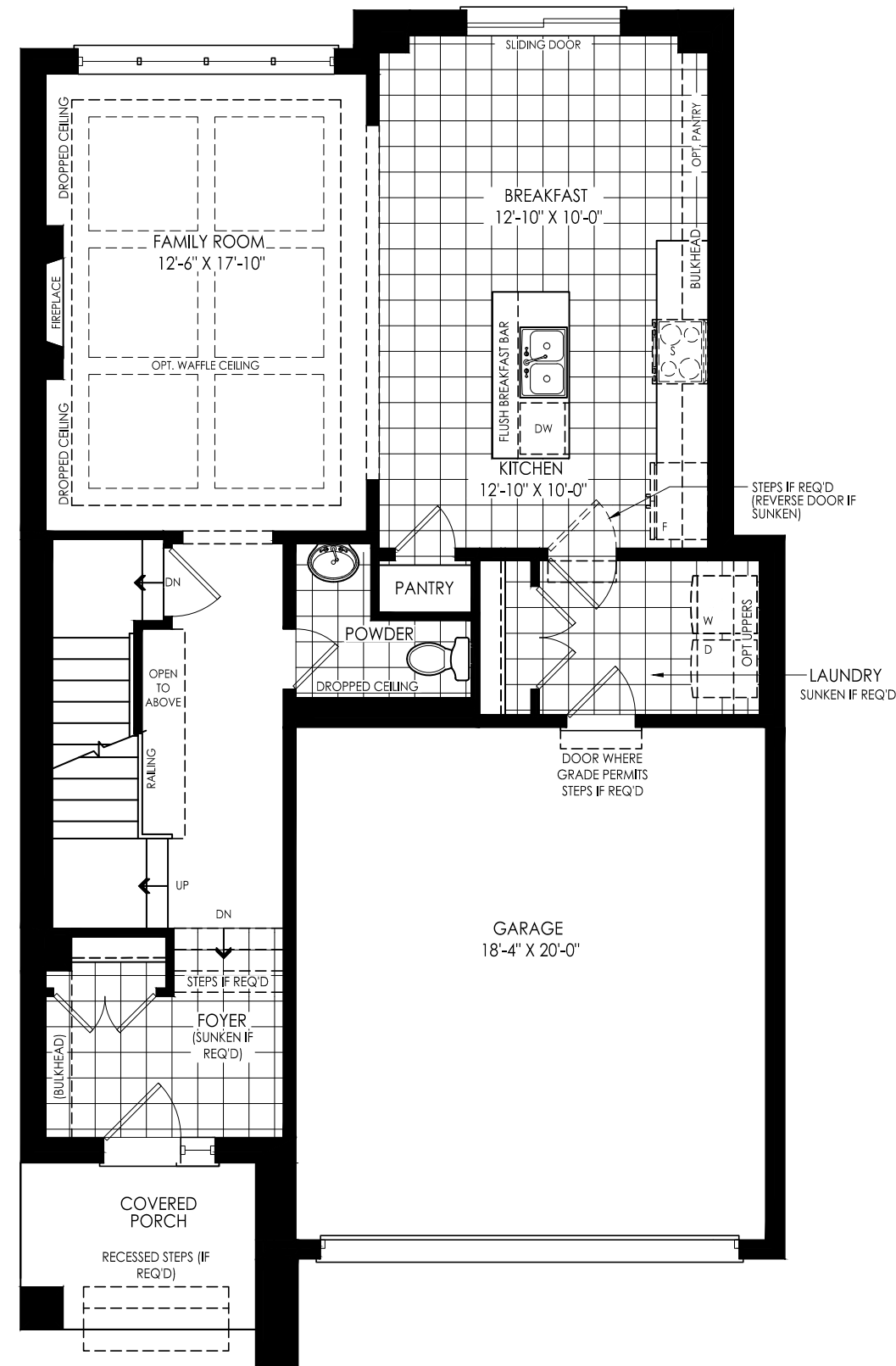
GROUND FLOOR PLAN ELEVATION D
