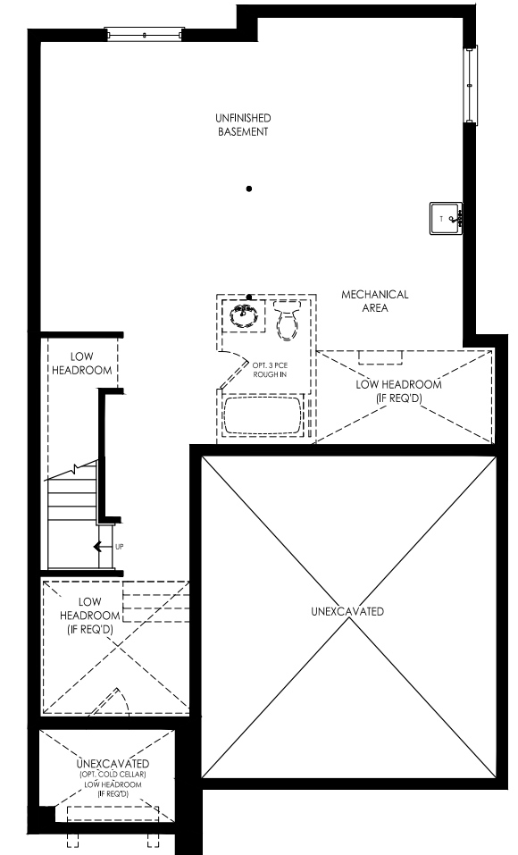
BASEMENT FLOOR PLAN ELEVATION D
