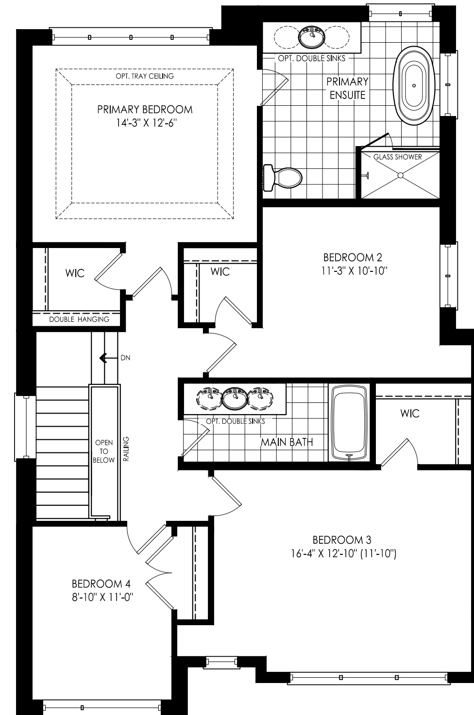
SECOND FLOOR PLAN ELEVATION D
