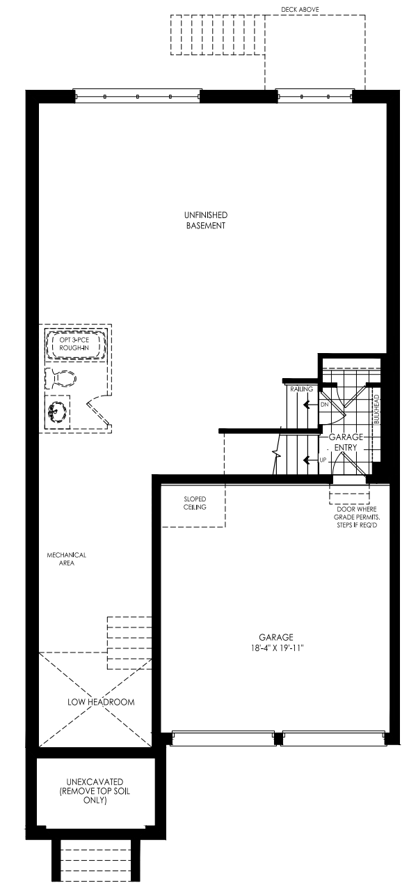
BASEMENT FLOOR PLAN ELEVATION C
