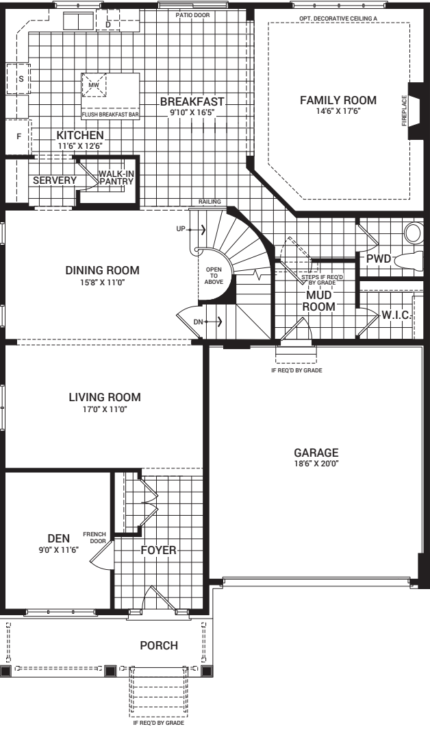
MAIN FLOOR
