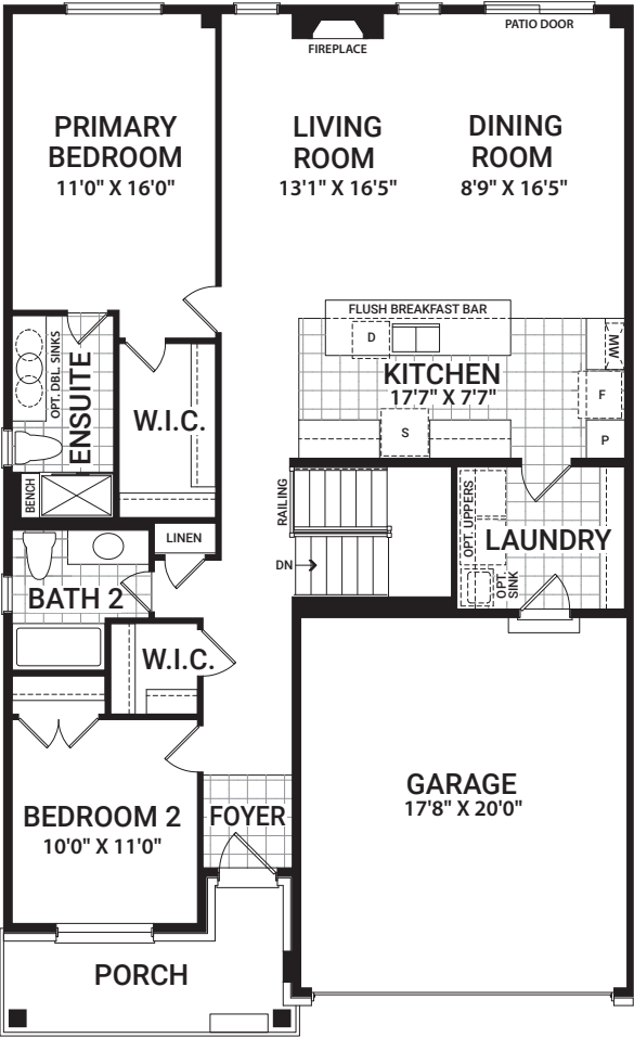
MAIN FLOOR
