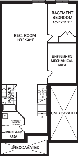
OPTIONAL FINISHED BASEMENT REC. ROOM W/BEDROOM
