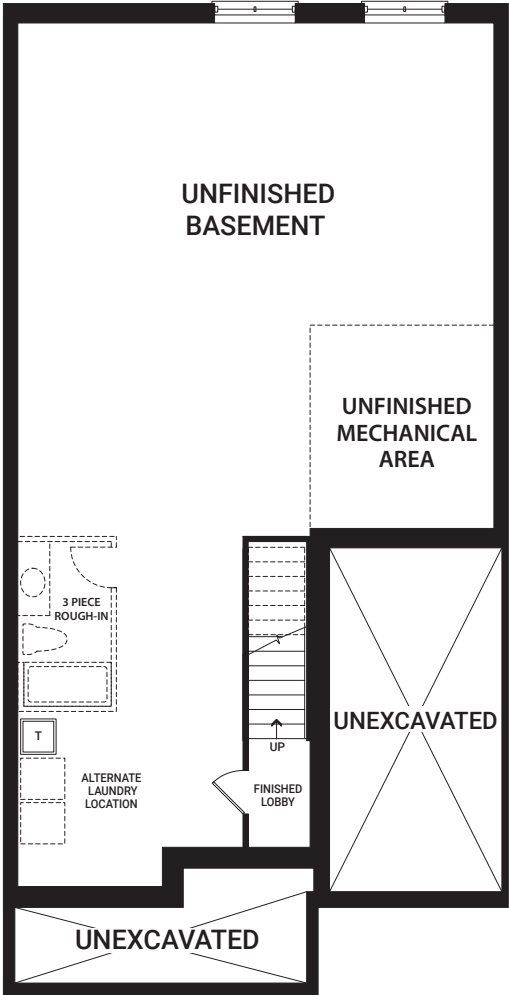
BASEMENT
