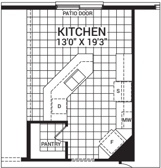
OPTIONAL KITCHEN LAYOUT A
