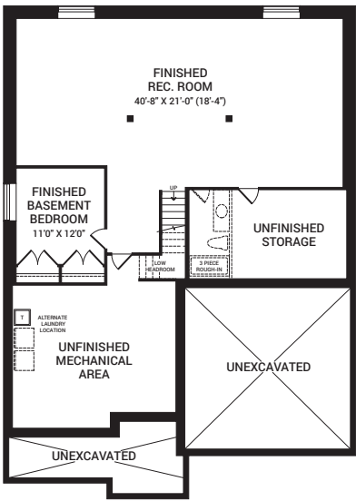
OPTIONAL FINISHED BASEMENT REC. ROOM W/BEDROOM
