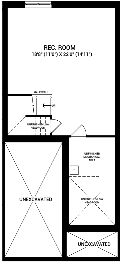
FINISHED BASEMENT
