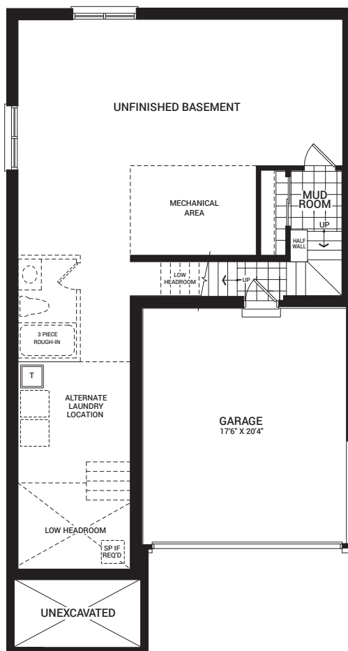
BASEMENT
