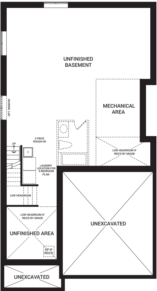
BASEMENT
