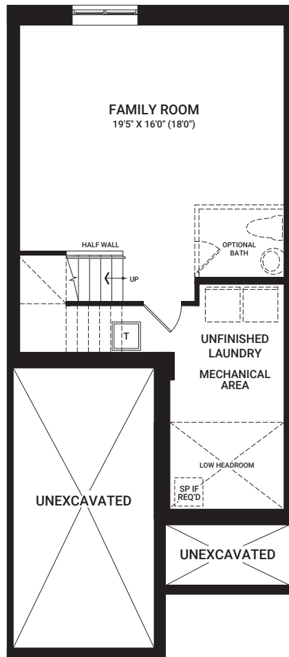
BASEMENT
