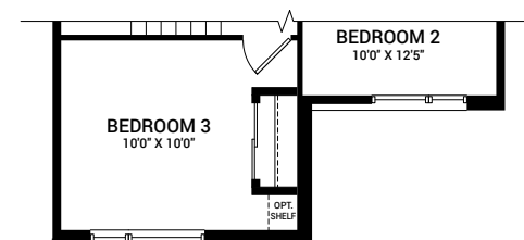
SECOND FLOOR PLAN D
