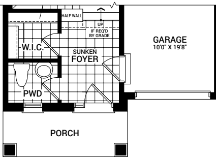
MAIN FLOOR PLAN B
