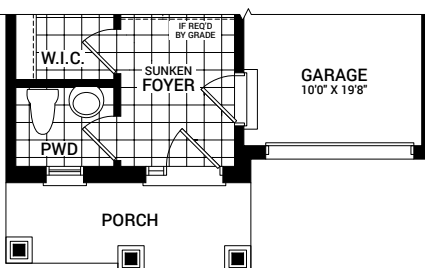
MAIN FLOOR PLAN C
