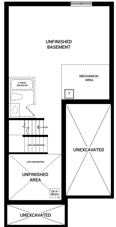
BASEMENT FLOOR PLAN A (SIMILAR FOR PLAN B, C & D)
