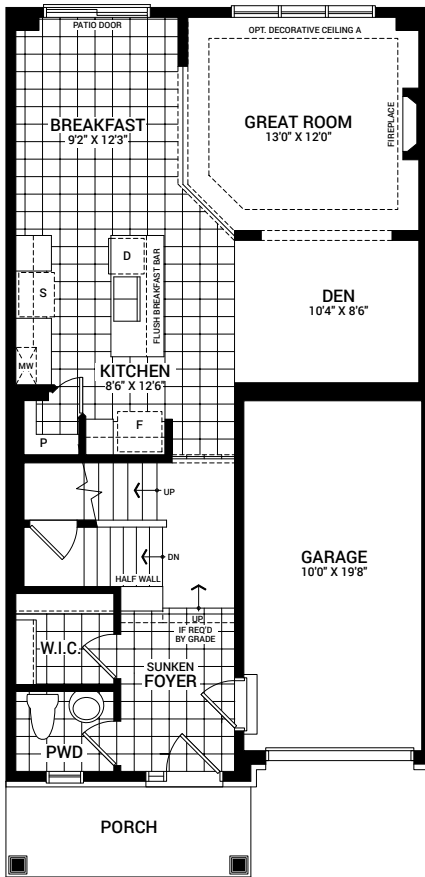
MAIN FLOOR PLAN A
