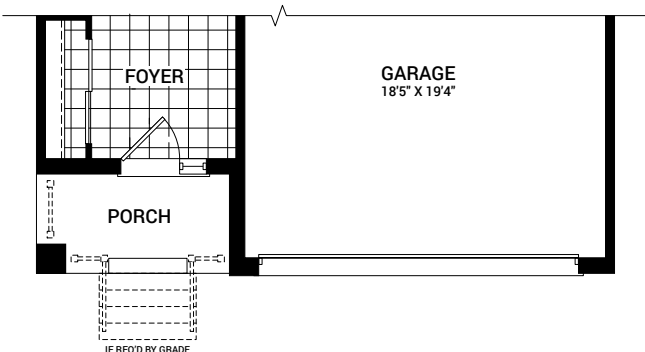
MAIN FLOOR PLAN D
